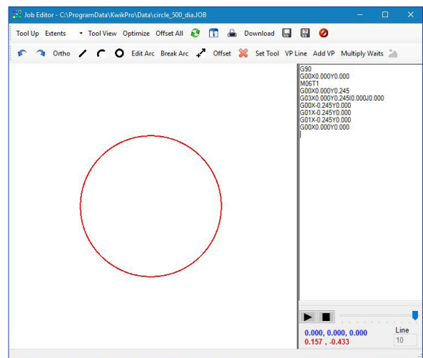
Simple G Code program defining the path
